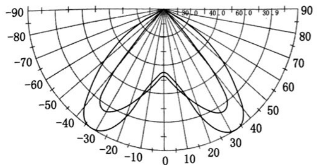
EMD Wide lens (Door Way)
